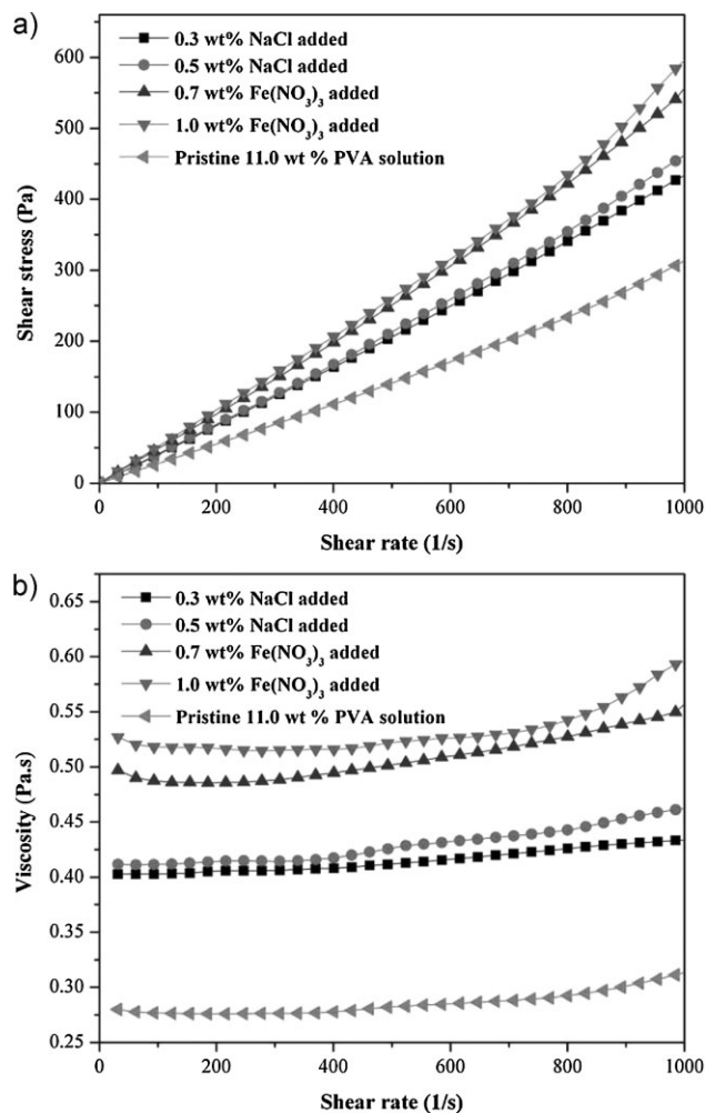
Figure 11. Rheological behavior analysis for (a) shear stress and (b) viscosity vs. shear rate of pristine PVA, PVA/NaCl, and PVA/ \text{Fe}(\text{NO}_3)_3 solution with different salt loadings.
