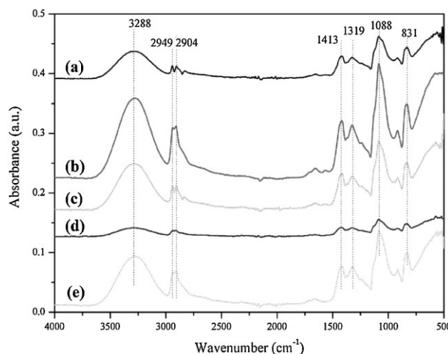
Figure 10. FT-IR spectra of (a) pristine PVA, (b) PVA/NaCl with 0.3 wt.-%, (c) 0.5 wt.-% loading, (d) PVA/ \text{Fe}(\text{NO}_3)_3 with 0.7 wt.-% and (e) 1.0 wt.-% loading nanocomposite fibers.
